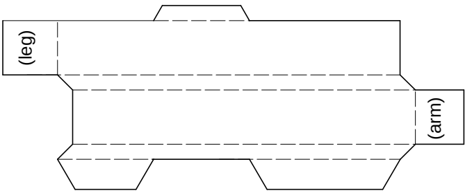
Arm Pushrod
