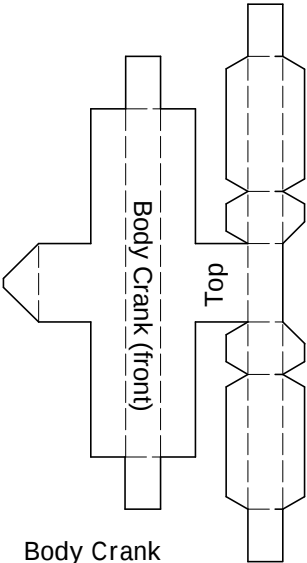
Body Crank
